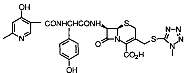
cefpiramide
